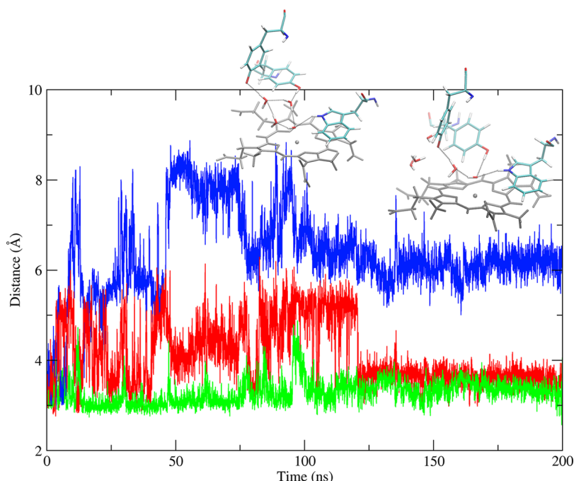
Figure 7. MD simulation showing structural rearrangements over 200 ns of the heme cavity of WT Tf-trHb at alkaline pH, following YB10 deprotonation, of the HO–O YB10 (blue), OH–N WG8 (green), and OH–O YCD1 (red) distances.
